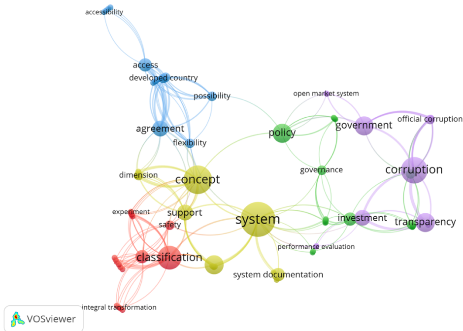
Figure 10. Keywords connectivity
