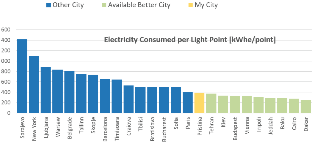
Diagram4 / Peer City Benchmark for Electricity consumed per Light Pole
